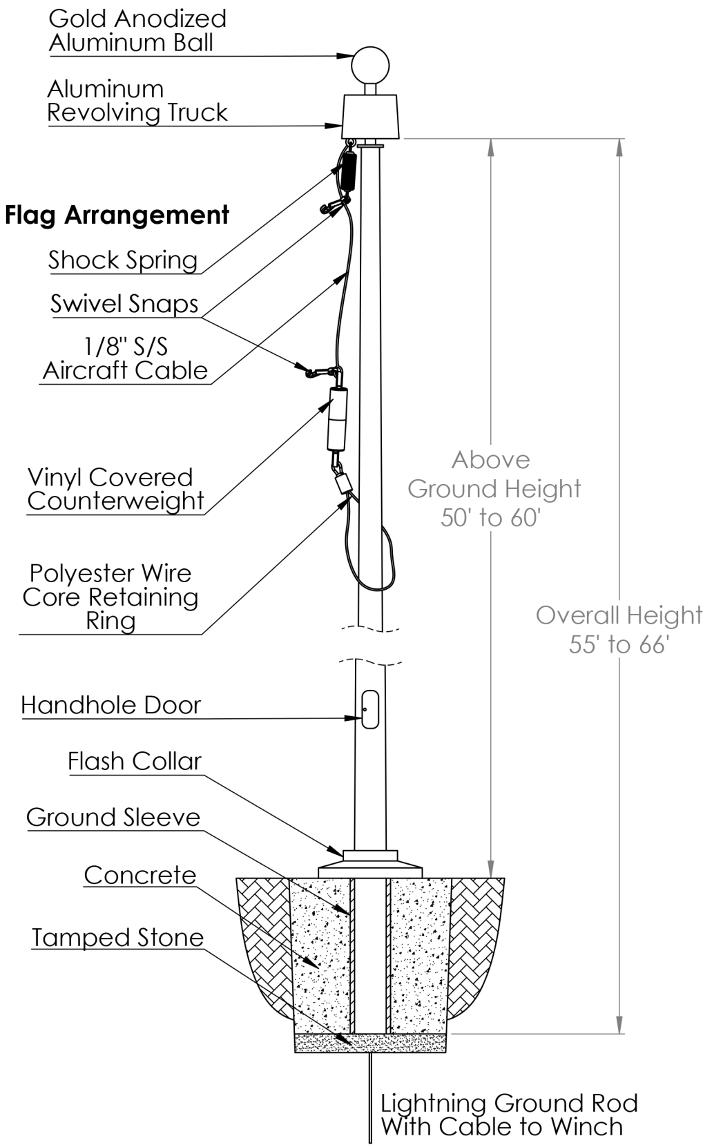
Internal Winch and Handhole Door
